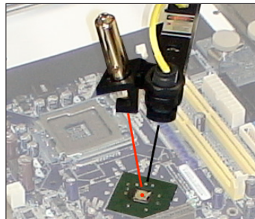
Temperature Sensor/Laser Pointer
